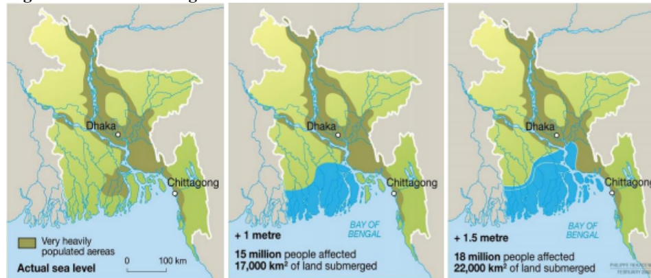
Figure 1: Land submerged in case of a 1.0 or 1.5 meter sea-level rise
